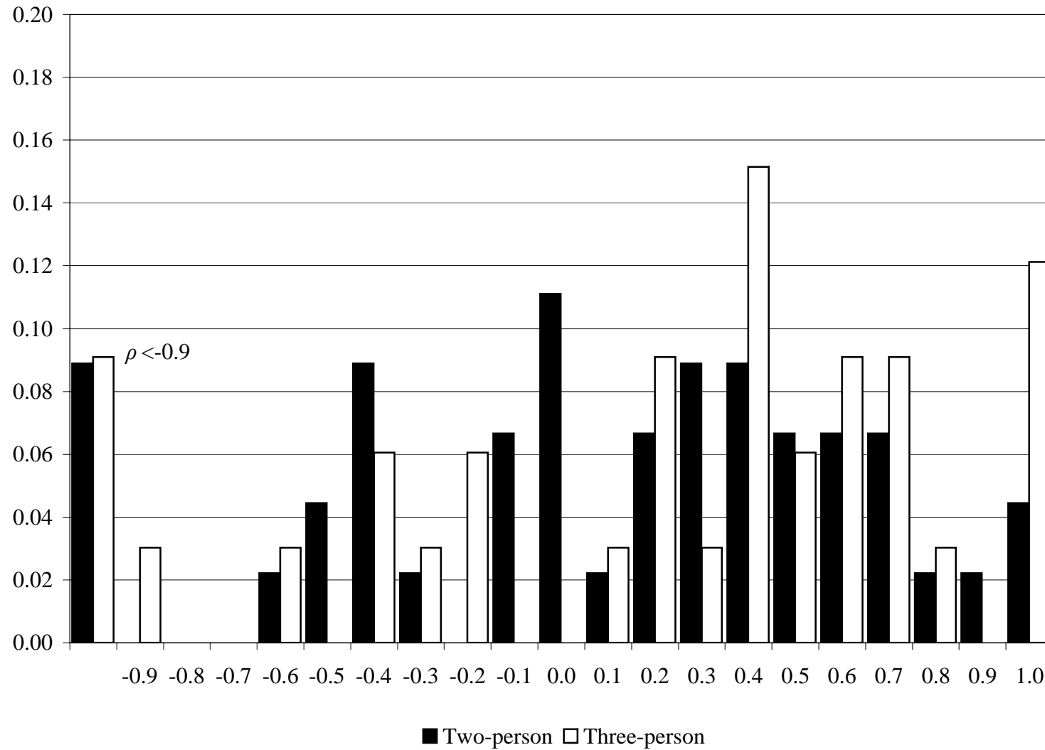
Figure 7: The distribution of the CES parameter \rho in the two- and three-person budget set experiments
